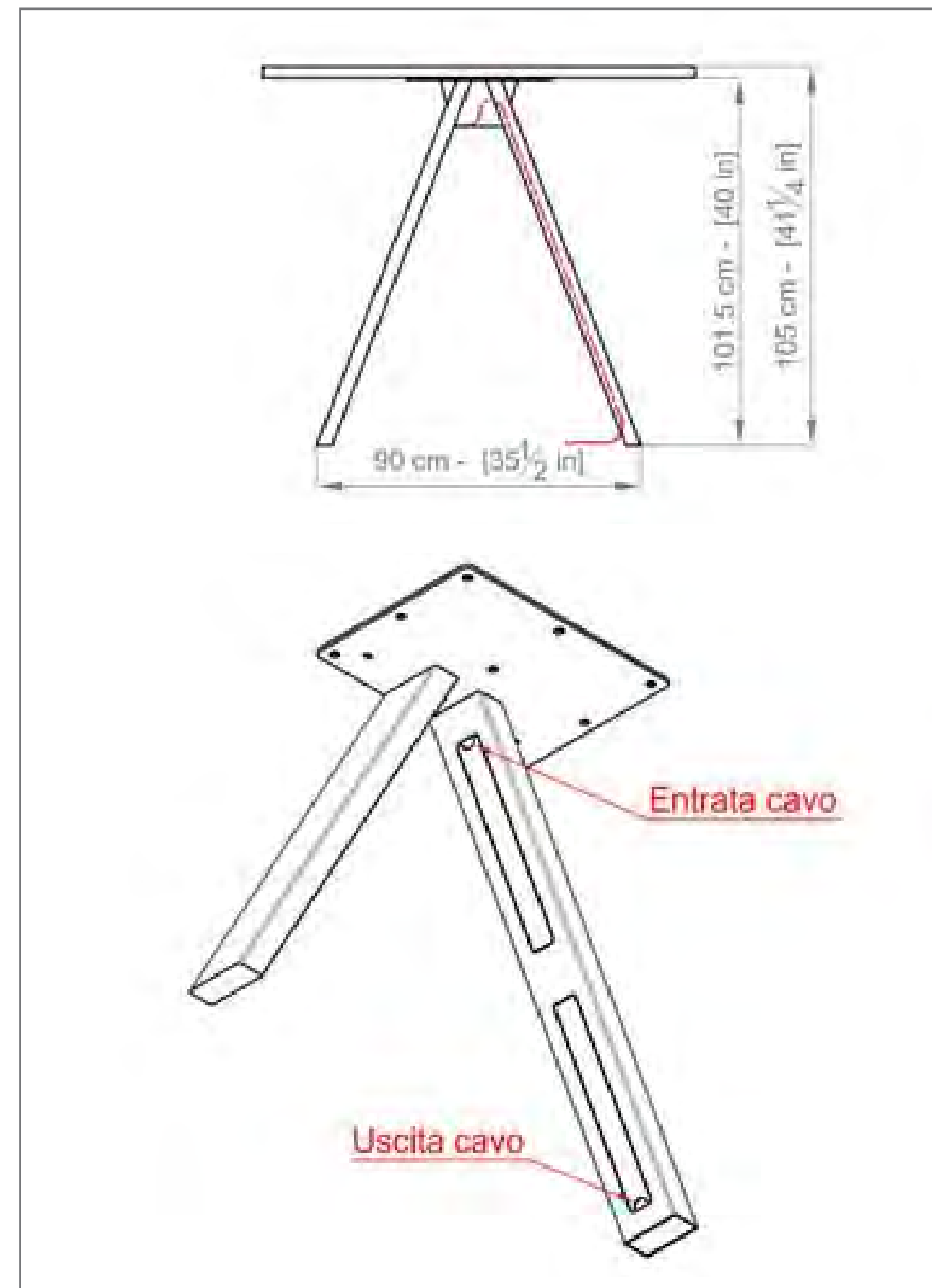
CROSS | LEG ELECTRIFICATION
